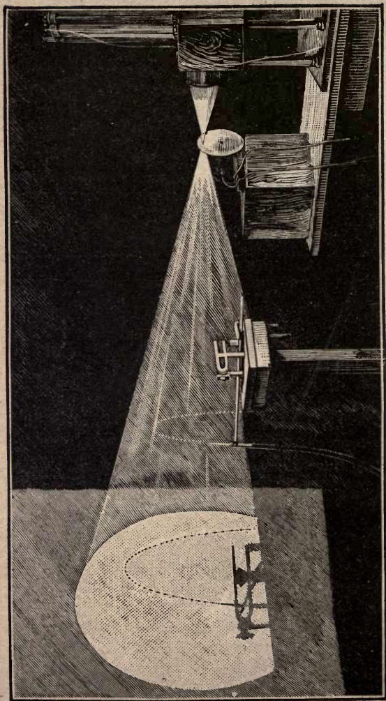
Experiment for showing by intermittent light the apparently stationary drops into which a fountain is broken up by the action of a musical sound. (See page 109.)
