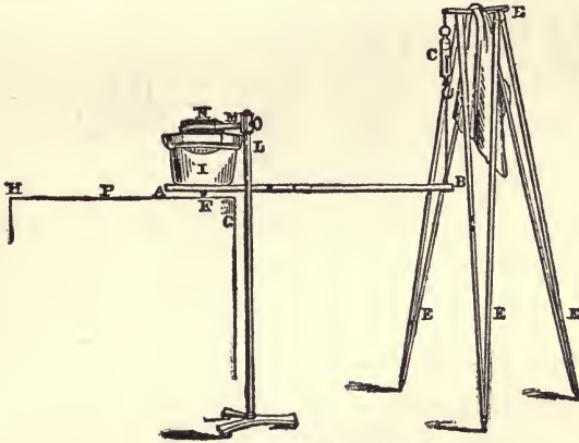
FIG. 9. CROOKES' APPARATUS.
