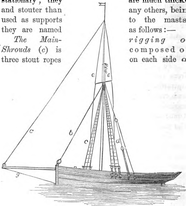
STANDING RIGGING.
