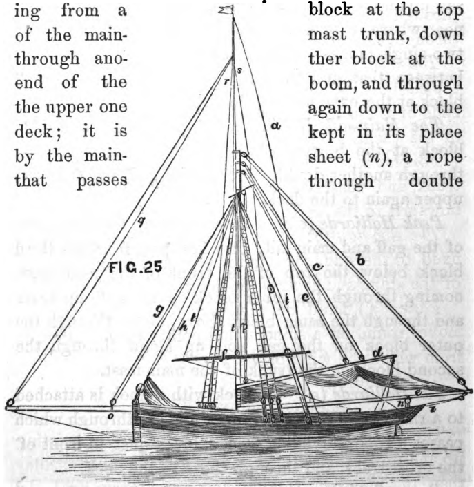
RUNNING RIGGING.
