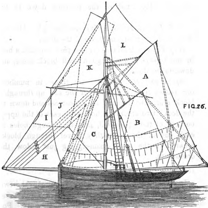
THE SAILS.
