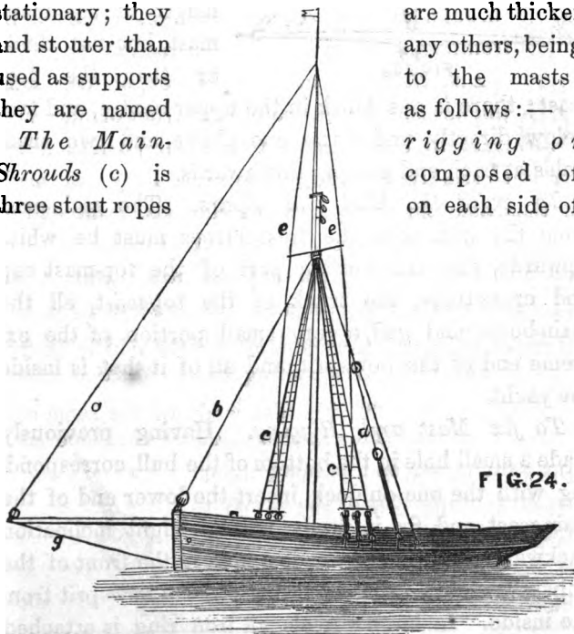
STANDING RIGGING.
